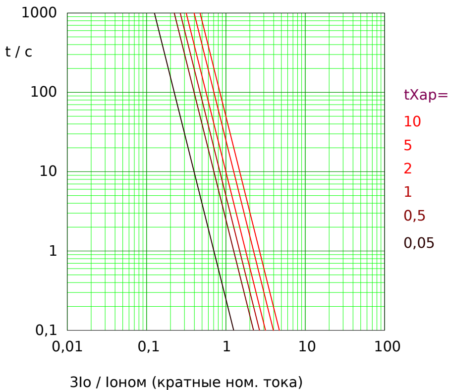
Рис. 79: I4T tripping curve. Note that only the range 3I_o \geq 3I_o> is actually effective.
