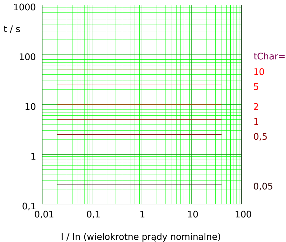
Rys. 72: Termiczna Płaska tripping curve. Note that only the range I \geq I > is actually effective.
