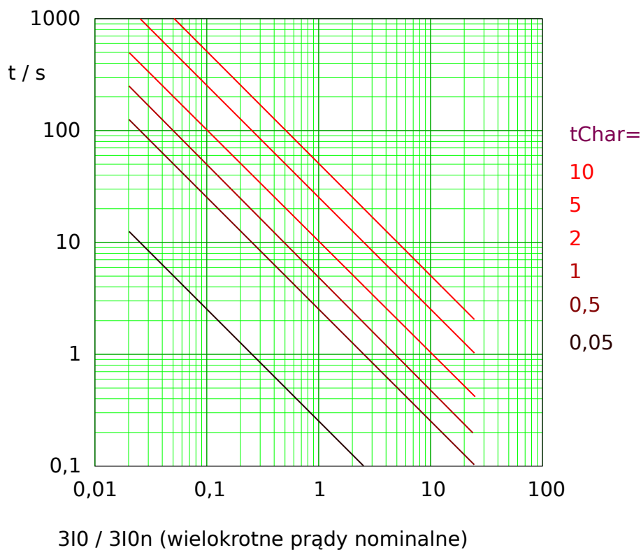
Rys. 77: IT tripping curve. Note that only the range 3I0 \geq \text{Próg } 3I0 is actually effective.
