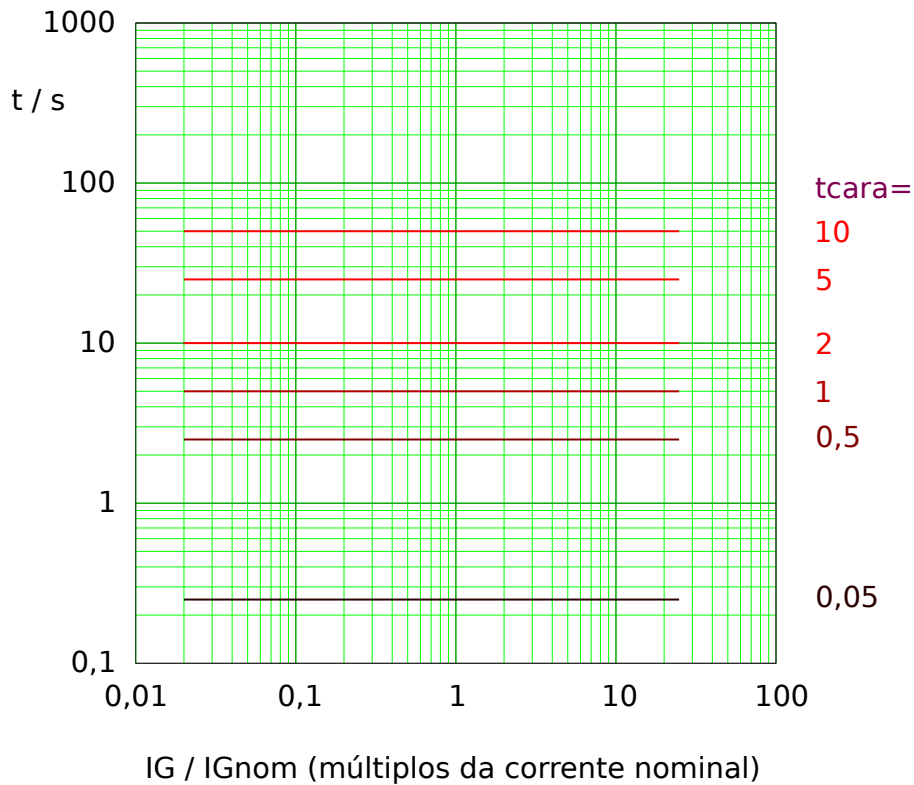
Fig. 76: Sup Térm tripping curve. Note that only the range IG \geq IG> is actually effective.
