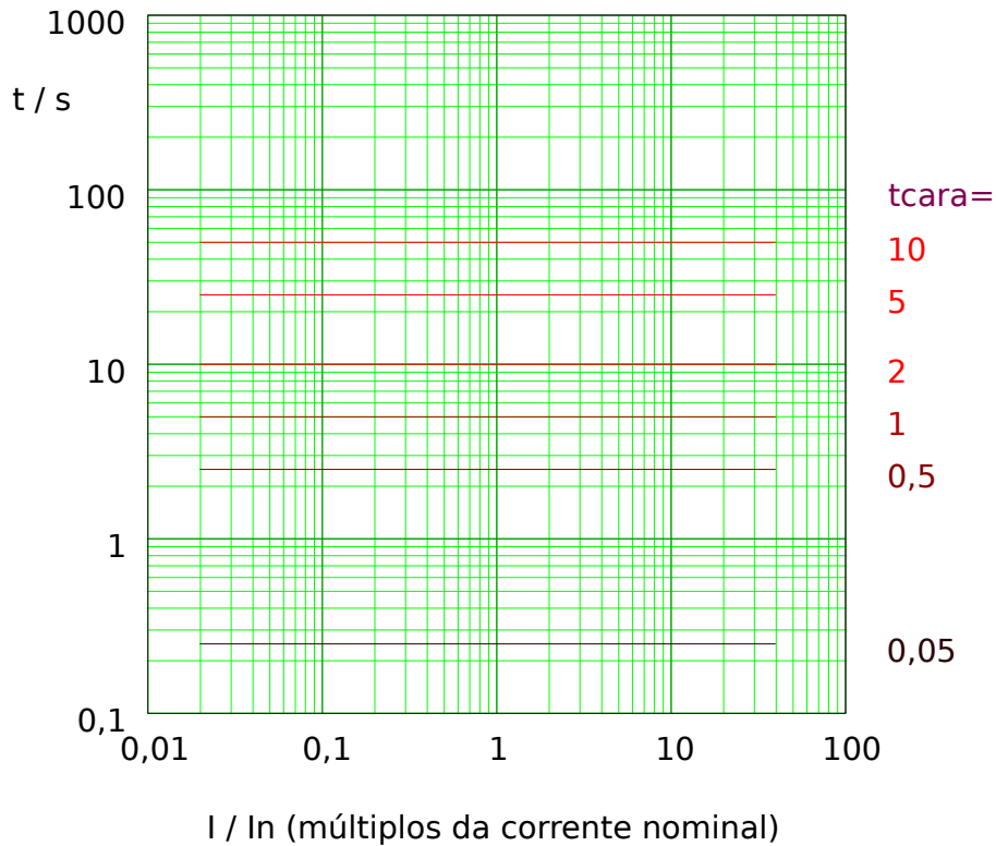
Fig. 72: Sup Térm tripping curve. Note that only the range I \geq I> is actually effective.
