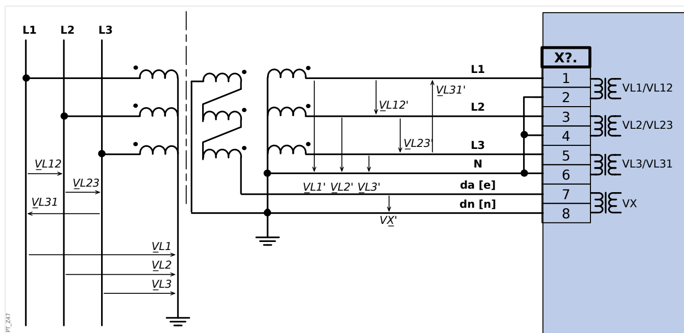
Fig. 29: VT Wye com conexão Broken Delt.
