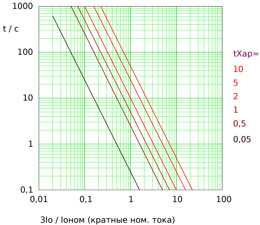
Рис. 68: I2T tripping curve. Note that only the range 3I_o \geq 3I_o> is actually effective.
