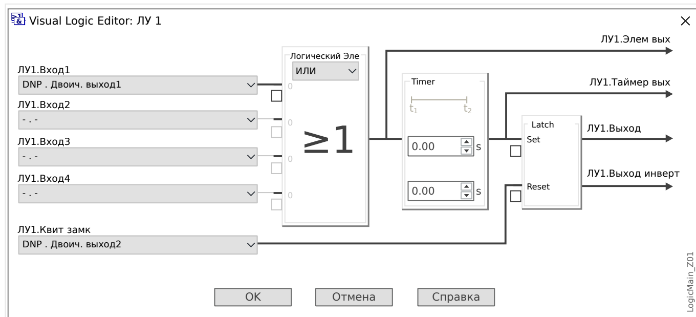
Рис. 46: Setting example from Smart view, to make a steady state signal from a DNP output signal.
