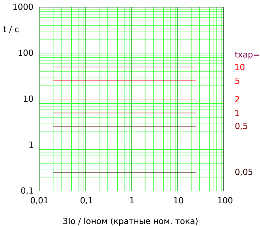
Рис. 66: Thermal Flat tripping curve. Note that only the range 3I_0 \geq 3I_0> is actually effective.
