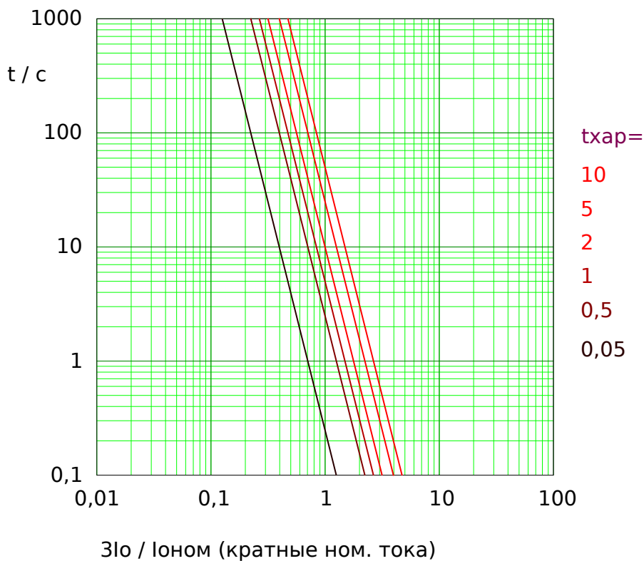
Рис. 69: I4T tripping curve. Note that only the range 3I_0 \geq 3I_0> is actually effective.
