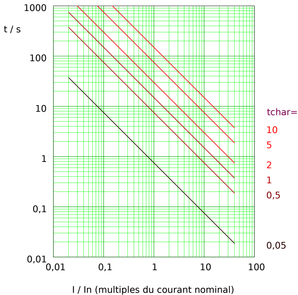
Fig. 63: IT tripping curve. Note that only the range I \geq I> is actually effective.
