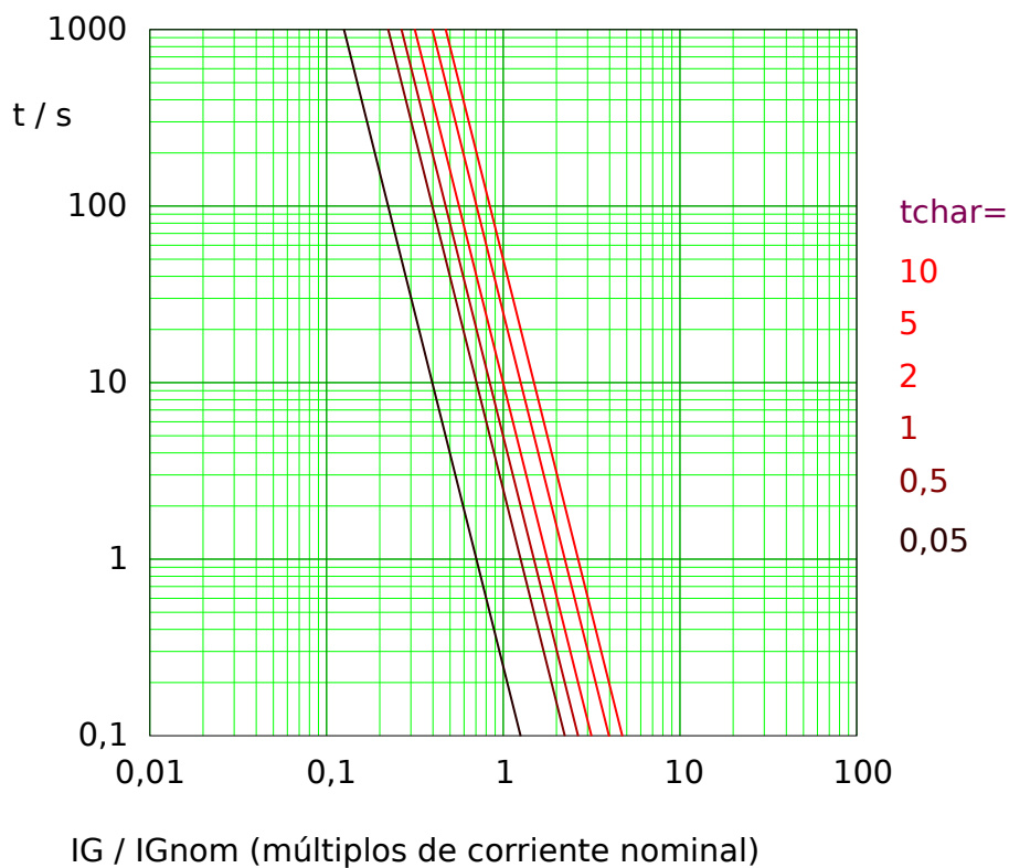
Fig. 69: I4T tripping curve. Note that only the range IG \geq IG_{nom} is actually effective.
