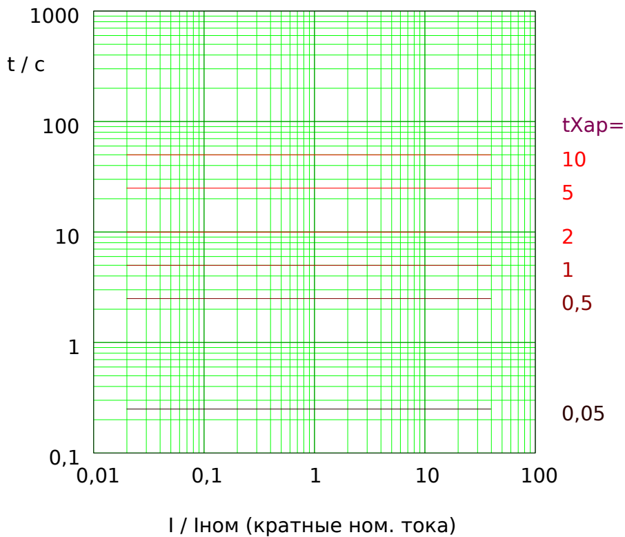
Рис. 45: Thermal Flat tripping curve. Note that only the range I \geq I> is actually effective.
