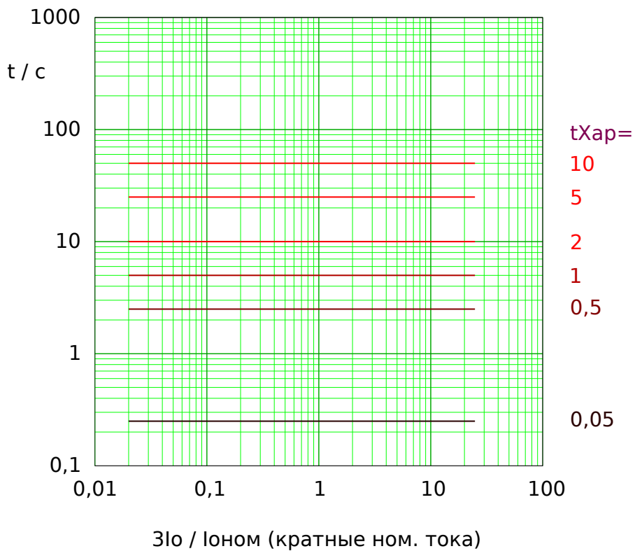
Рис. 49: Thermal Flat tripping curve. Note that only the range 3I_0 \geq 3I_0> is actually effective.
