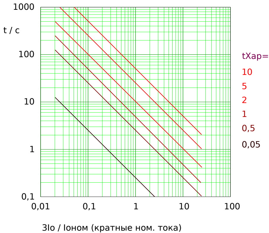
Рис. 50: IT tripping curve. Note that only the range 3I_o \geq 3I_o> is actually effective.
