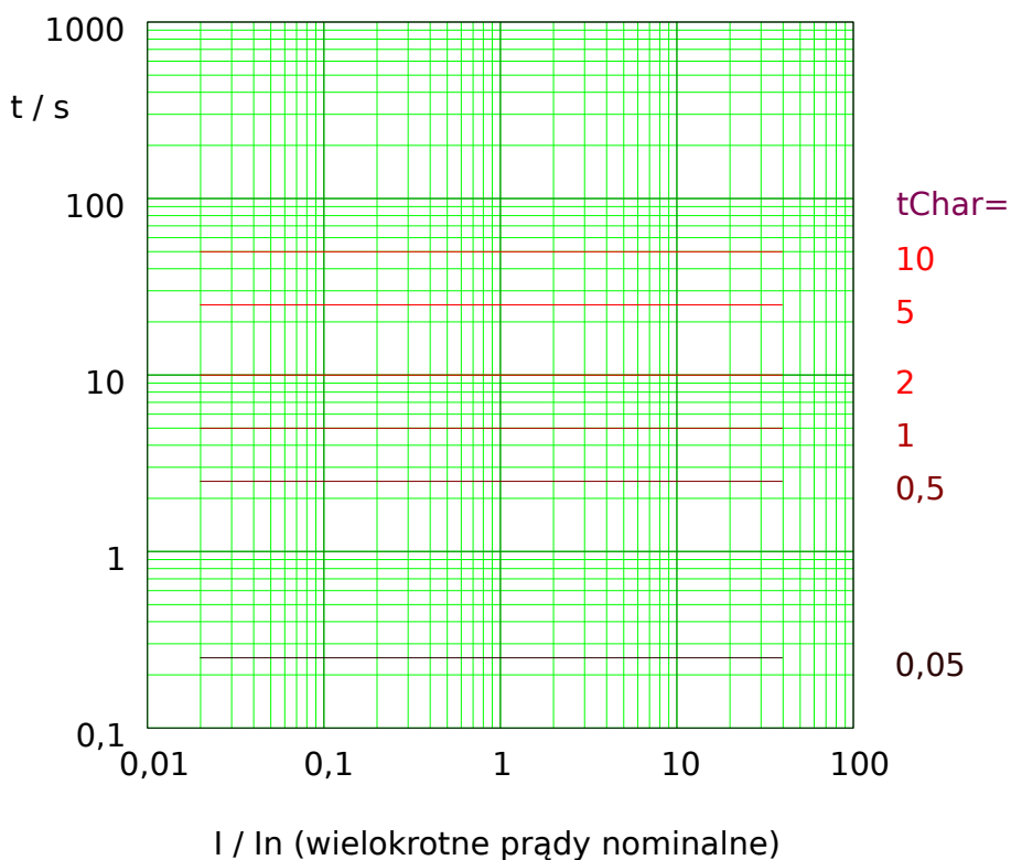
Rys. 45: Termiczna Płaska tripping curve. Note that only the range I \geq I> is actually effective.
