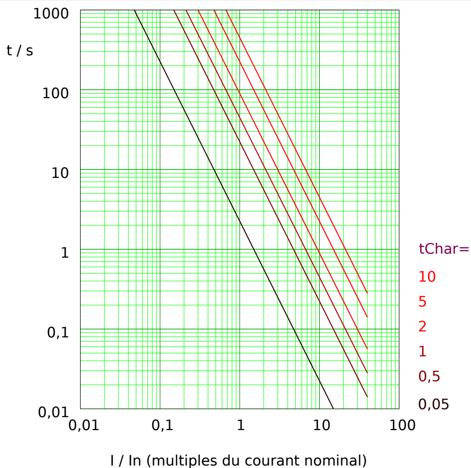
Fig. 47: I2T tripping curve. Note that only the range I \geq I_n is actually effective.
