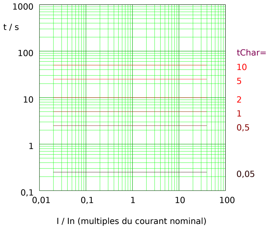
Fig. 45: Therm Flat tripping curve. Note that only the range I \geq I> is actually effective.
