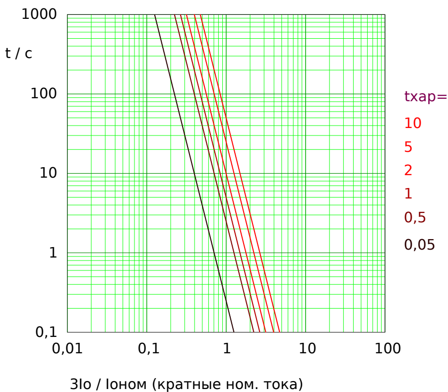
Рис. 52: I4T tripping curve. Note that only the range 3I_0 \geq 3I_0> is actually effective.
