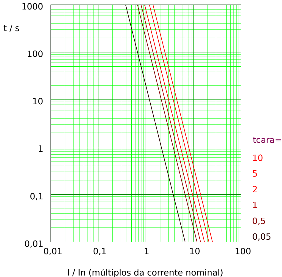
Fig. 48: I4T tripping curve. Note that only the range I \geq I_n is actually effective.
