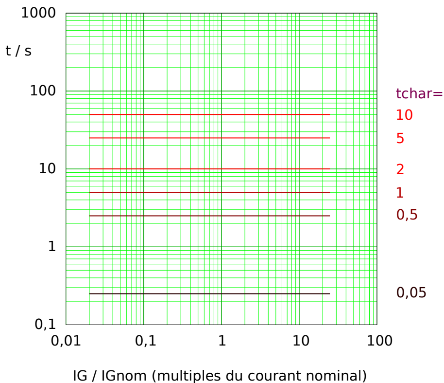
Fig. 49: Therm Flat tripping curve. Note that only the range IG \geq IG> is actually effective.
