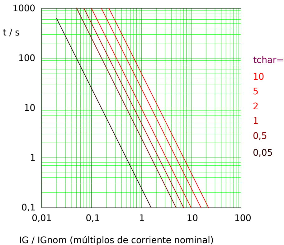
Fig. 51: I2T tripping curve. Note that only the range IG \geq IG_{nom} is actually effective.
