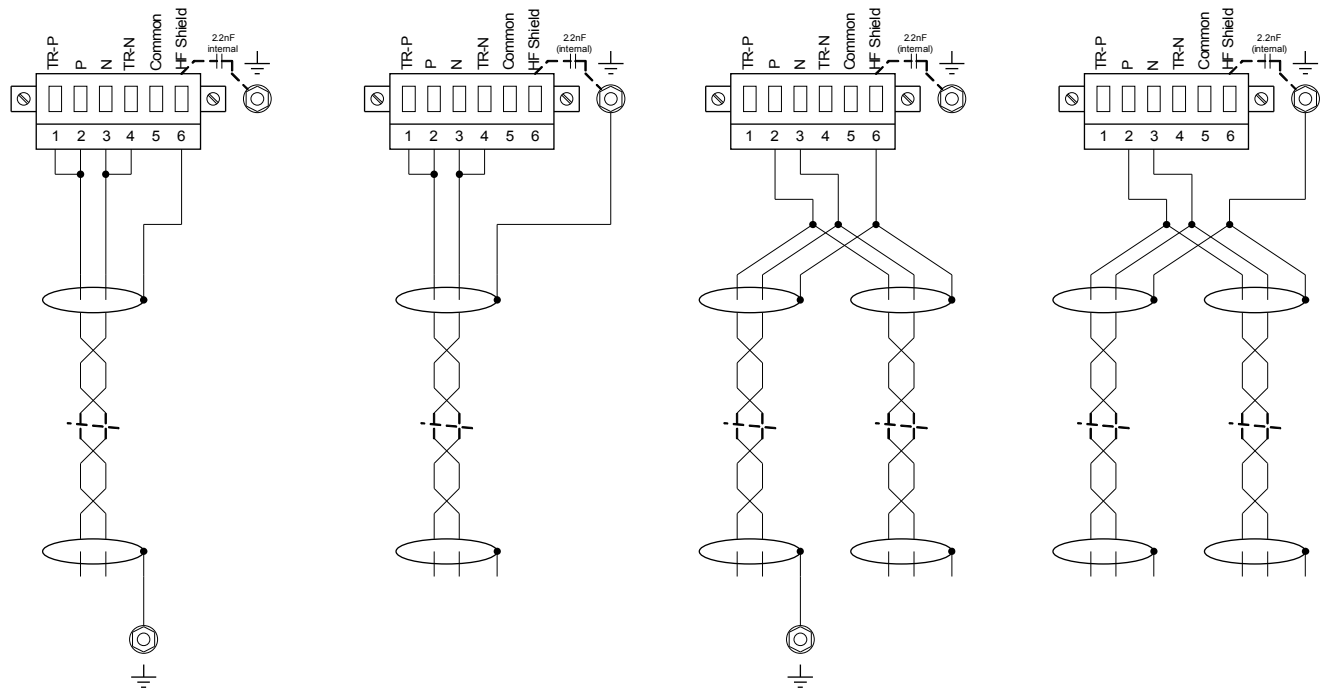
Shield at bus master side connected to earth termination resistors used
