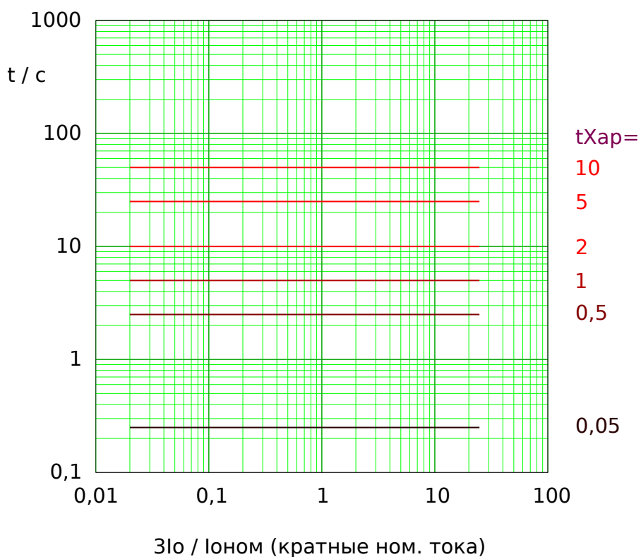
Рис. 58: Thermal Flat tripping curve. Note that only the range 3I_0 \geq 3I_0> is actually effective.
