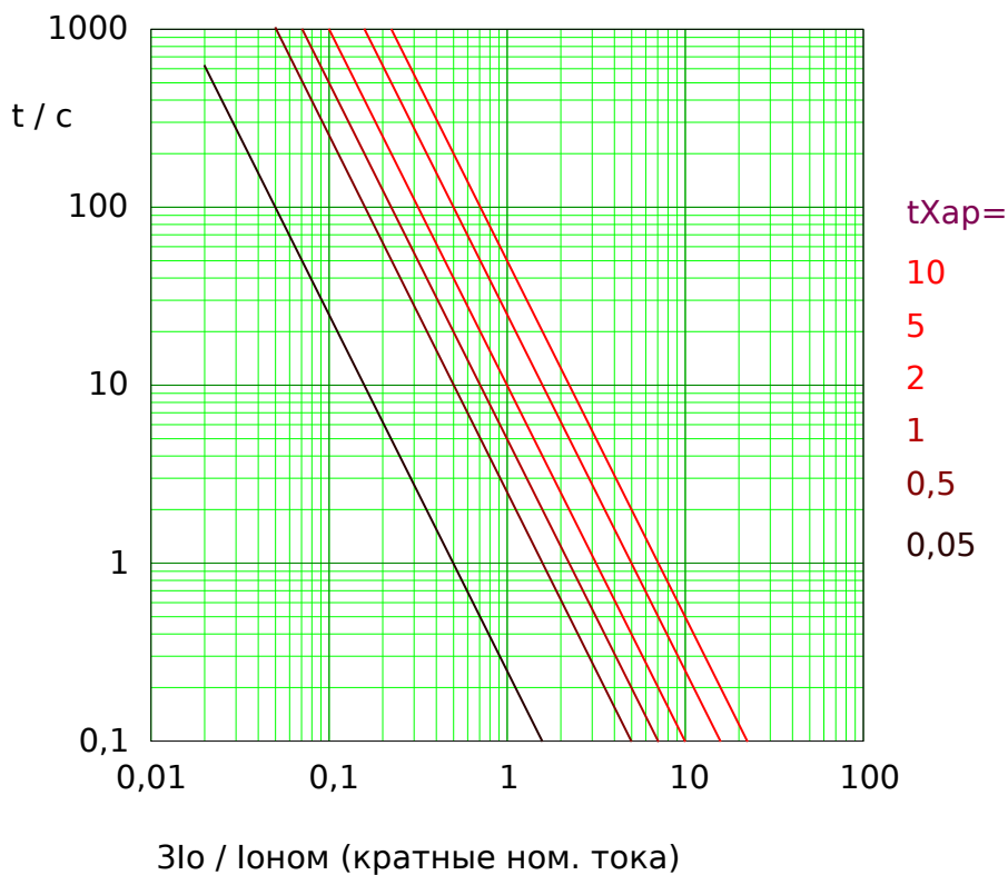
Рис. 60: I2T tripping curve. Note that only the range 3I_o \geq 3I_o> is actually effective.
