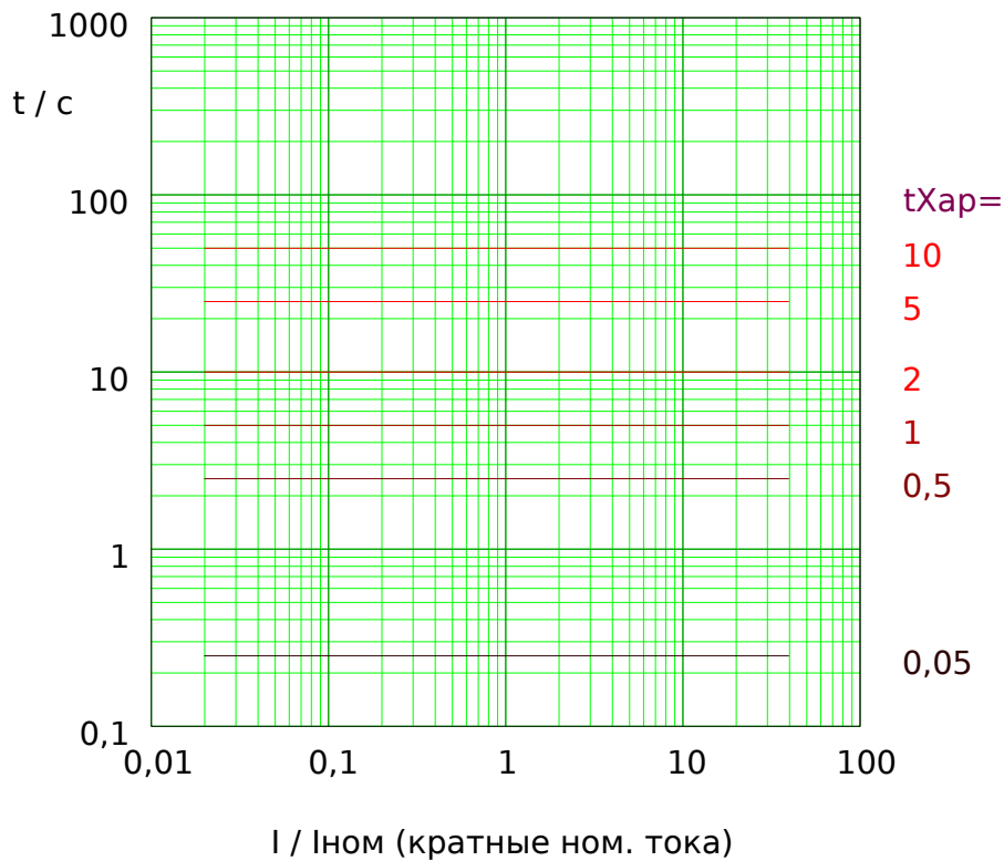
Рис. 54: Thermal Flat tripping curve. Note that only the range I \geq I> is actually effective.
