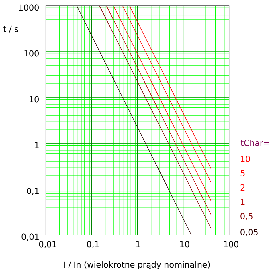
Rys. 56: I 2 T tripping curve. Note that only the range I \geq I_n is actually effective.
