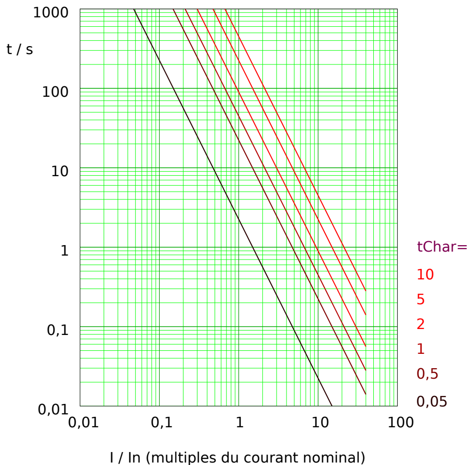
Fig. 56: I2T tripping curve. Note that only the range I \geq I> is actually effective.
