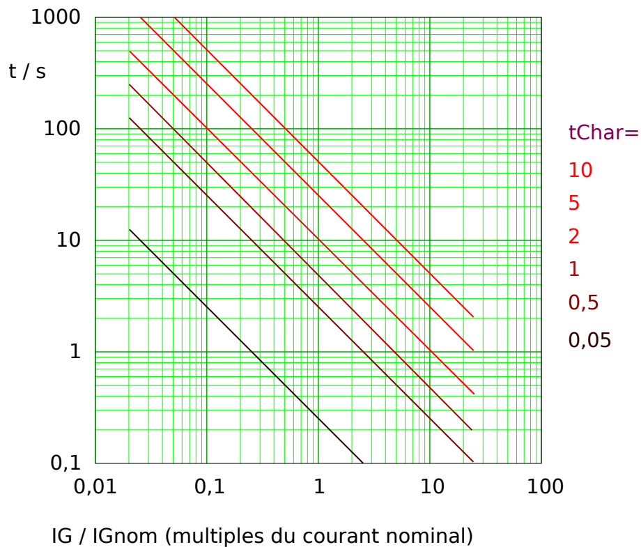
Fig. 59: IT tripping curve. Note that only the range IG \geq IG> is actually effective.
