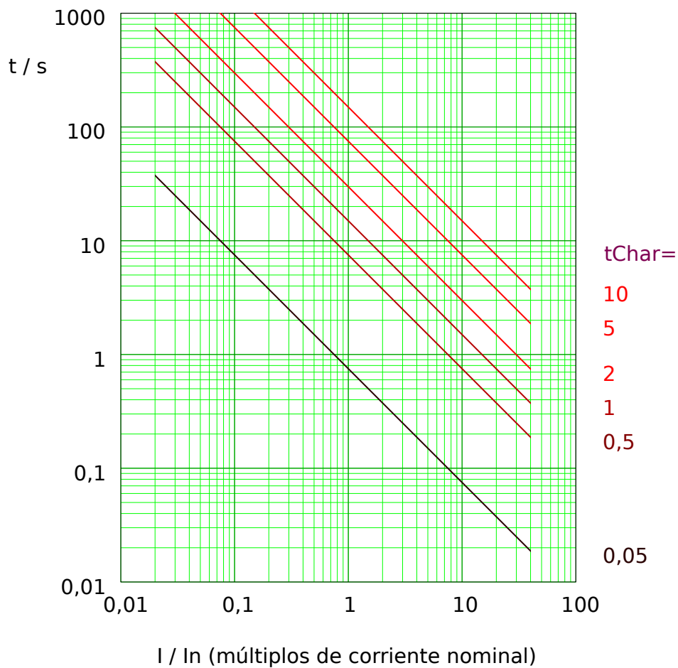
Fig. 55: IT tripping curve. Note that only the range I \geq I_n is actually effective.
