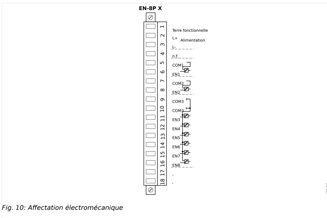
Fig. 9: Bornes
