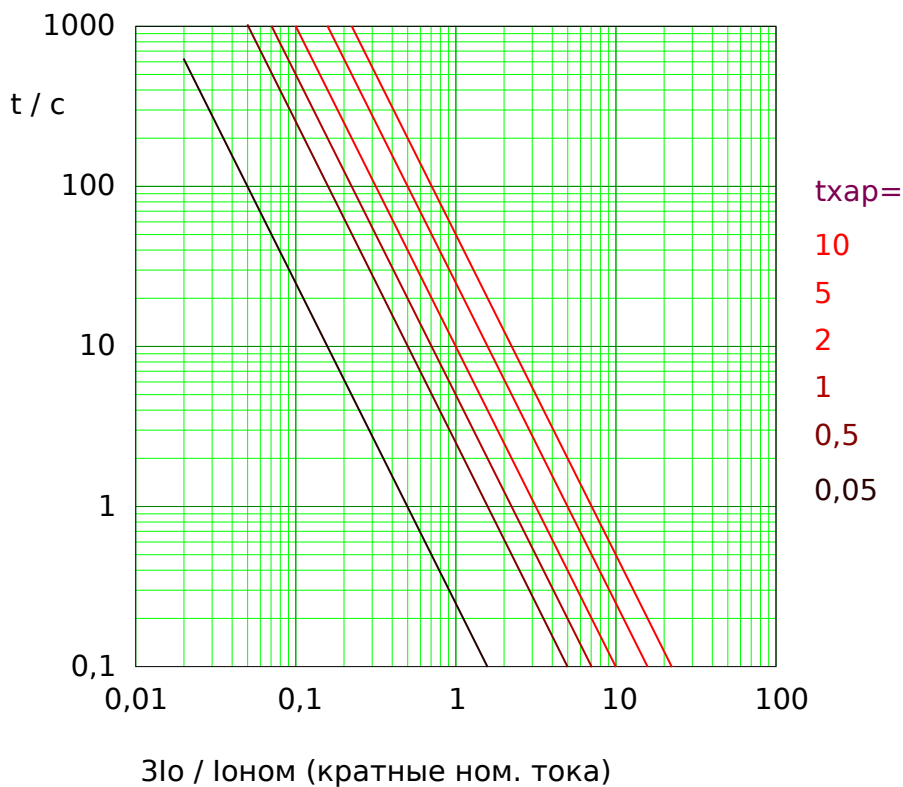
Рис. 60: I2T tripping curve. Note that only the range 3I_0 \geq 3I_0> is actually effective.
