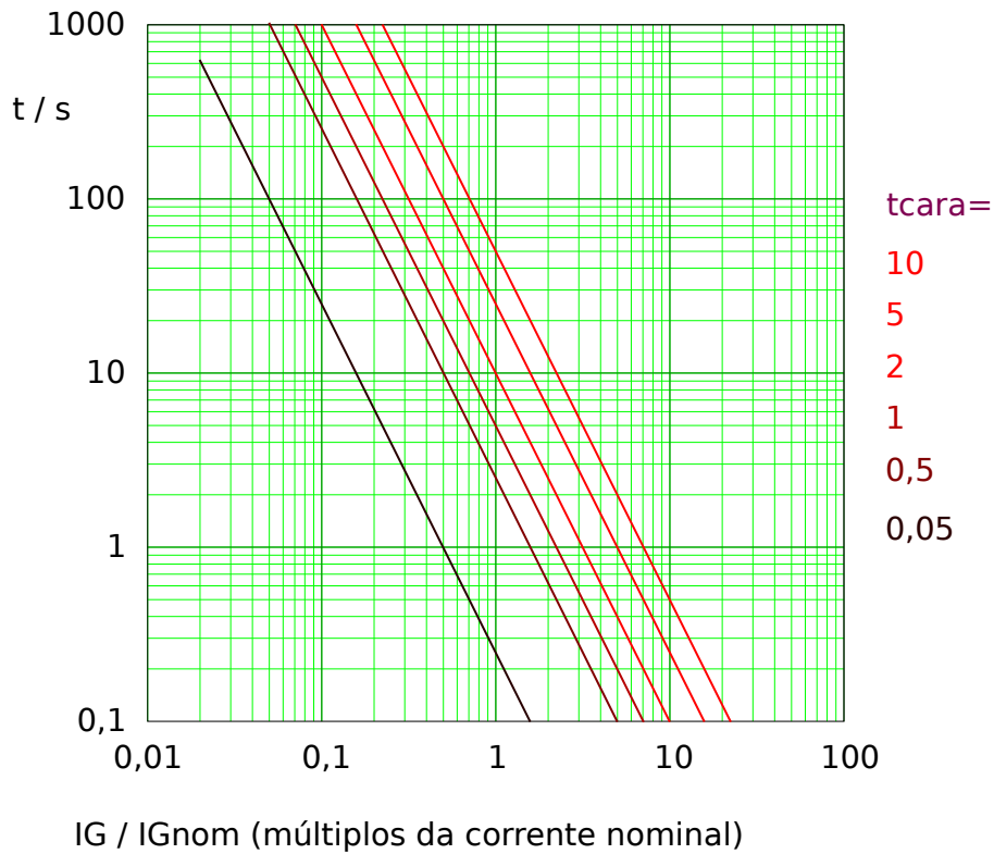
Fig. 60: I2T tripping curve. Note that only the range IG \geq IG_{>} is actually effective.
