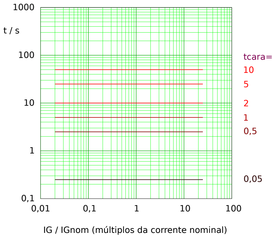
Fig. 58: Sup Térm tripping curve. Note that only the range IG \geq IG> is actually effective.
