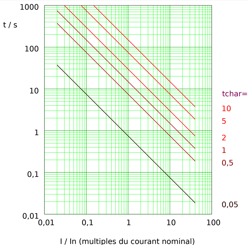
Fig. 55: IT tripping curve. Note that only the range I \geq I> is actually effective.
