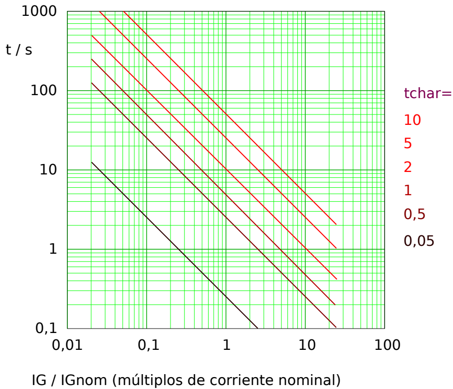
Fig. 59: IT tripping curve. Note that only the range IG \geq IG_{nom} is actually effective.
