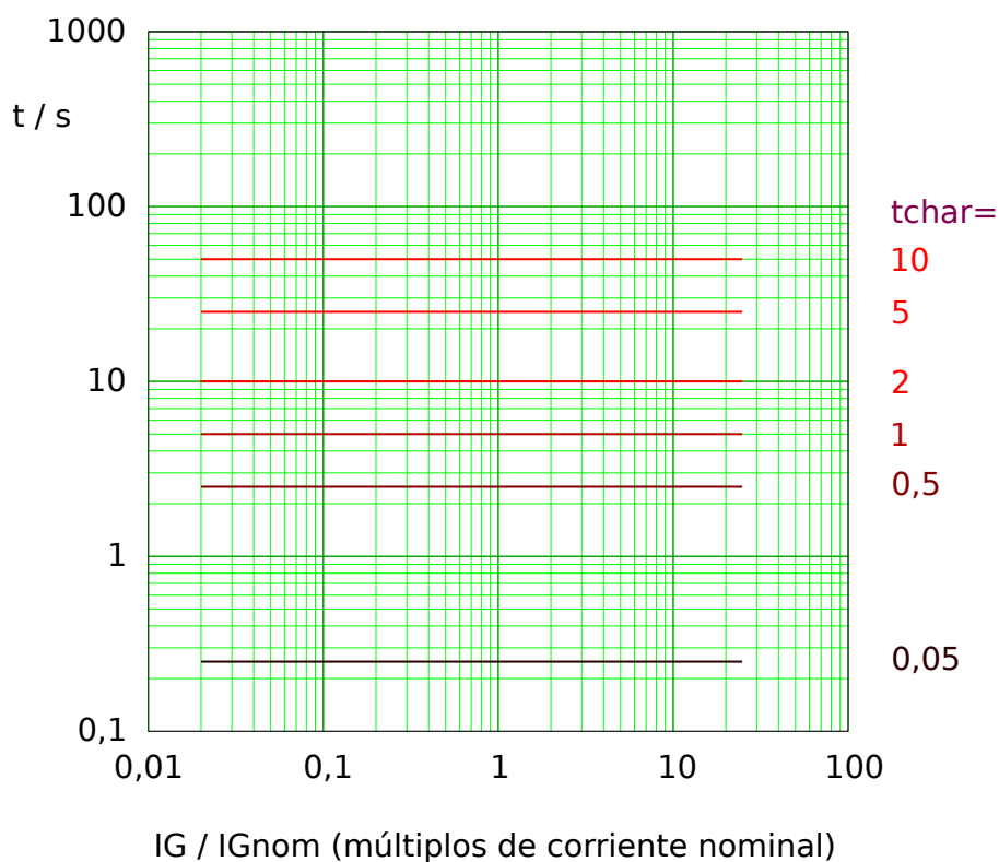
Fig. 58: Therm Flat tripping curve. Note that only the range IG \geq IG> is actually effective.
