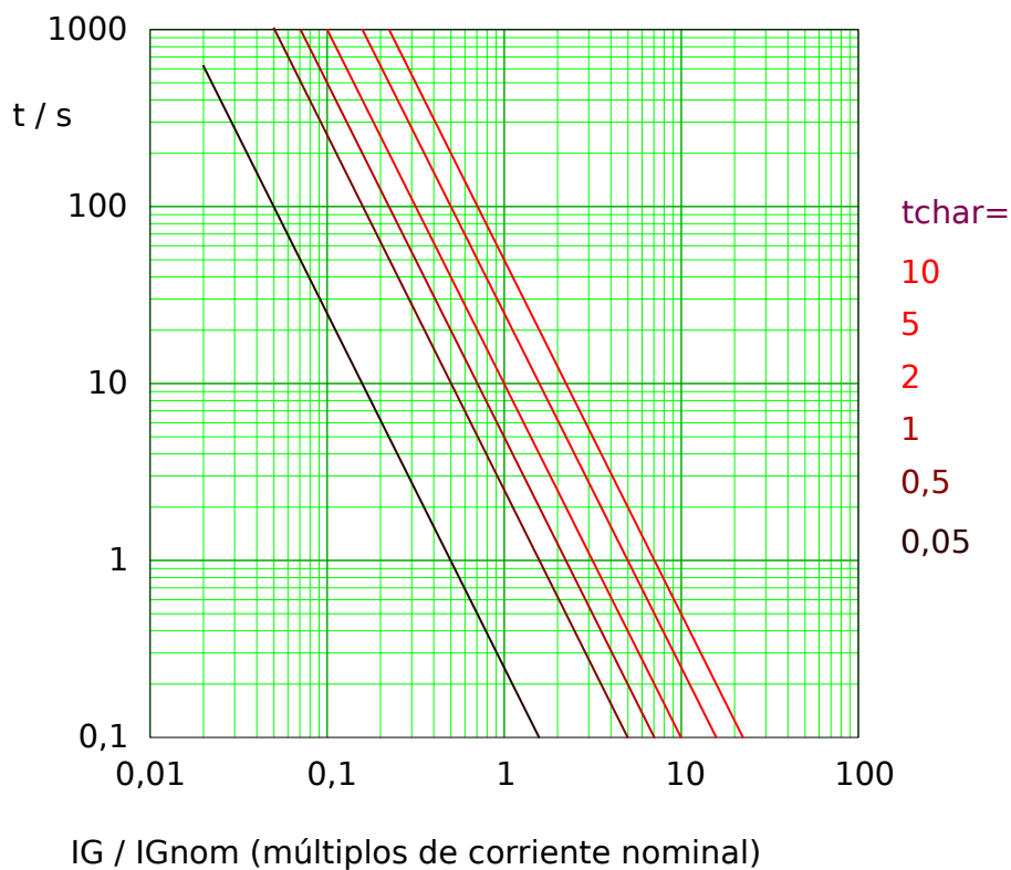
Fig. 60: I2T tripping curve. Note that only the range IG \geq IG_{nom} is actually effective.
