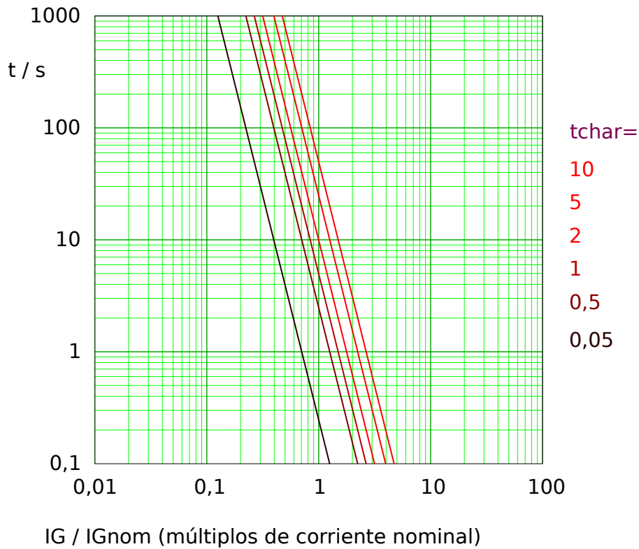
Fig. 61: I4T tripping curve. Note that only the range IG \geq IG_{>} is actually effective.
