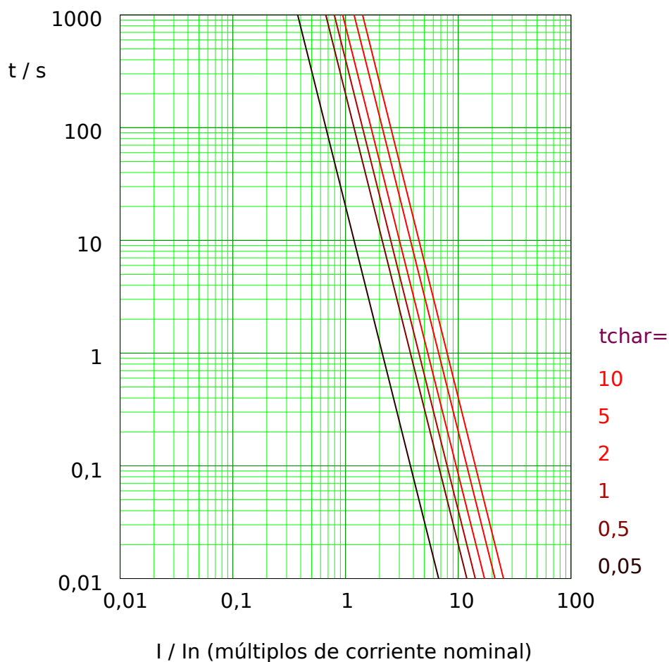
Fig. 57: I4T tripping curve. Note that only the range I \geq I> is actually effective.
