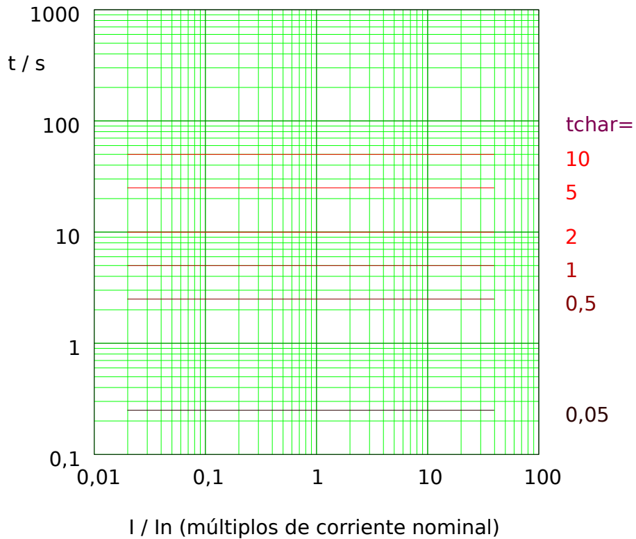
Fig. 54: Therm Flat tripping curve. Note that only the range I \geq I> is actually effective.
