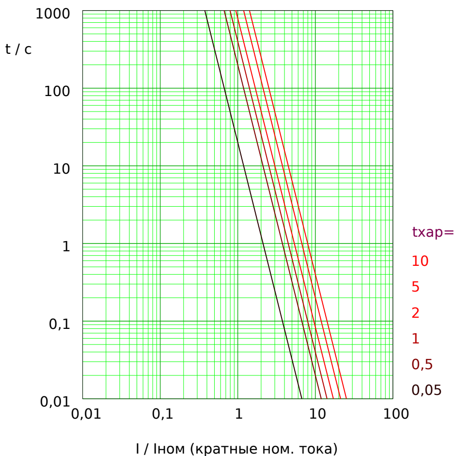
Рис. 74: I4T tripping curve. Note that only the range I \geq I > is actually effective.
