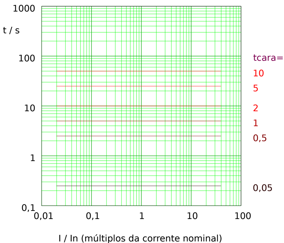
Fig. 71: Sup Térm tripping curve. Note that only the range I \geq I> is actually effective.
