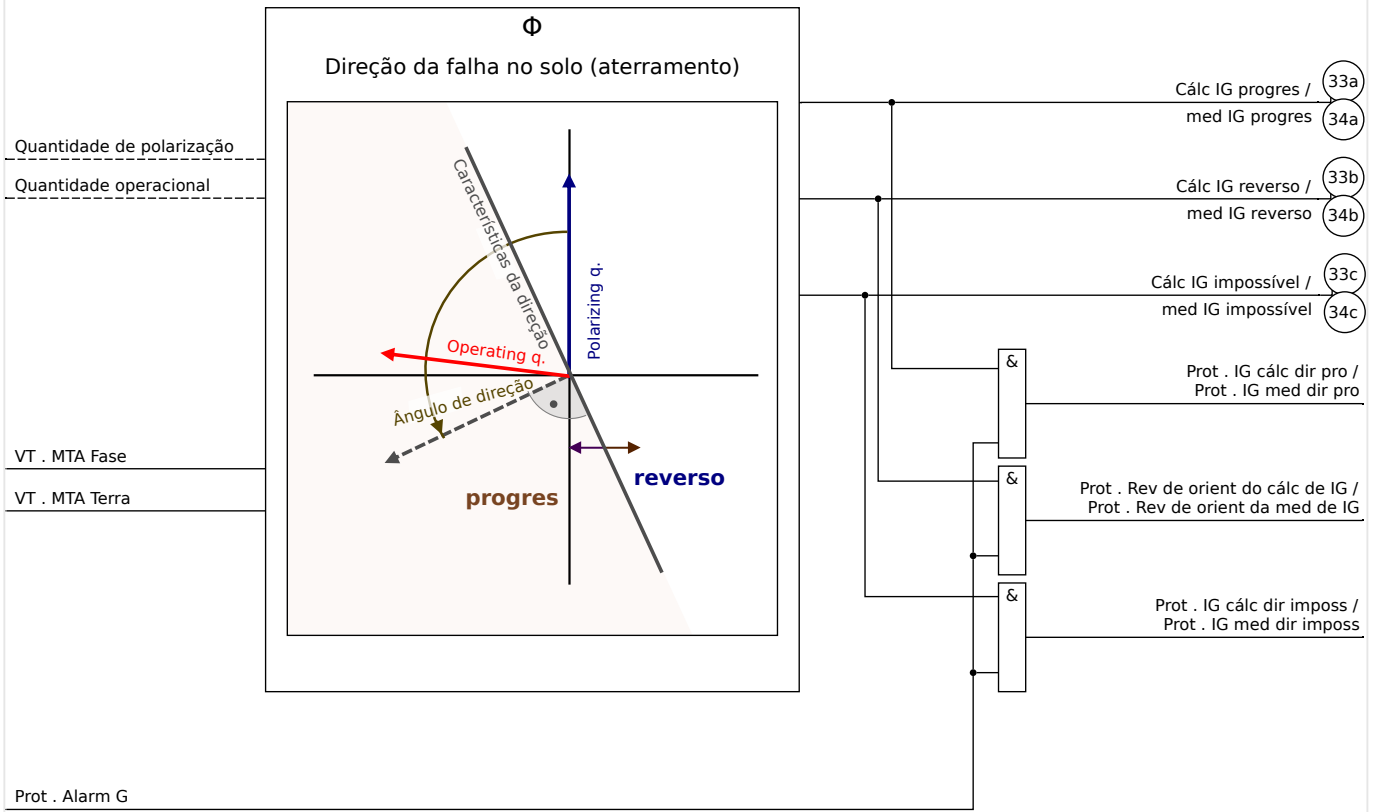
Fig. 67: Direction determination for all methods except "cos( \phi )", "sin( \phi )".
