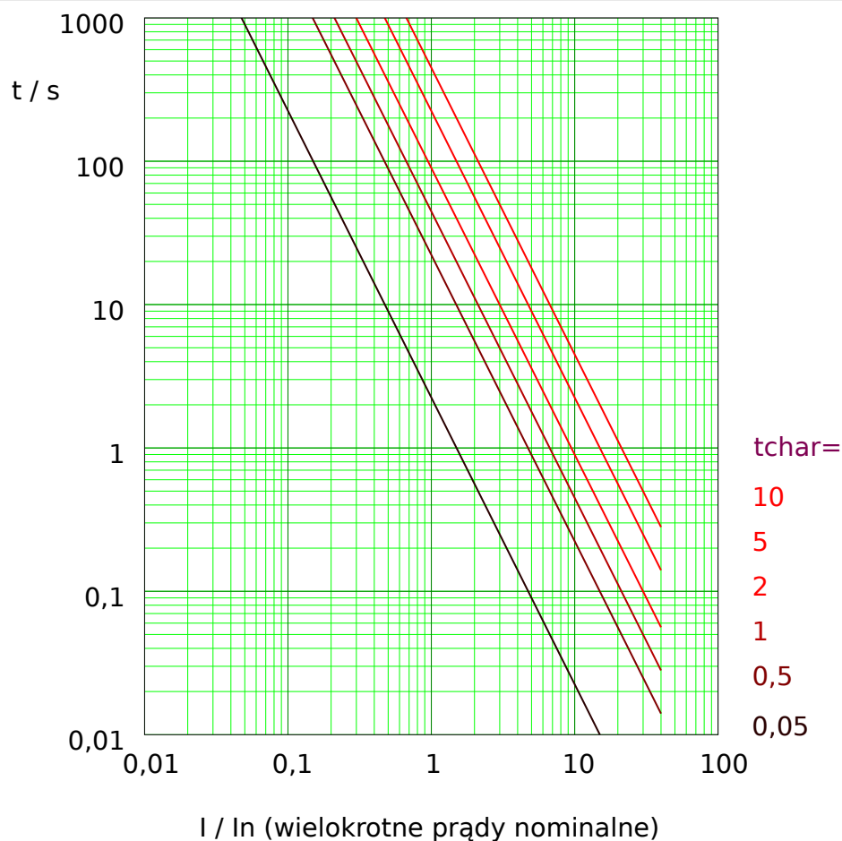
Rys. 83: I2T tripping curve. Note that only the range I \geq I_n is actually effective.
