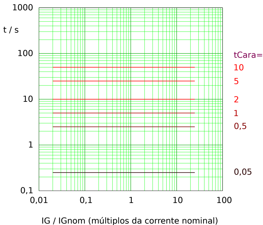
Fig. 89: Sup Térm tripping curve. Note that only the range IG \geq IG> is actually effective.
