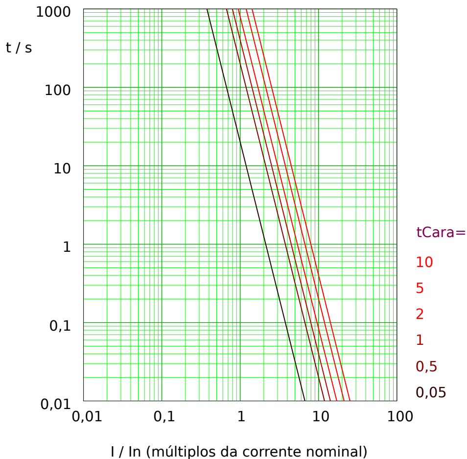
Fig. 88: I4T tripping curve. Note that only the range I \geq I_n is actually effective.
