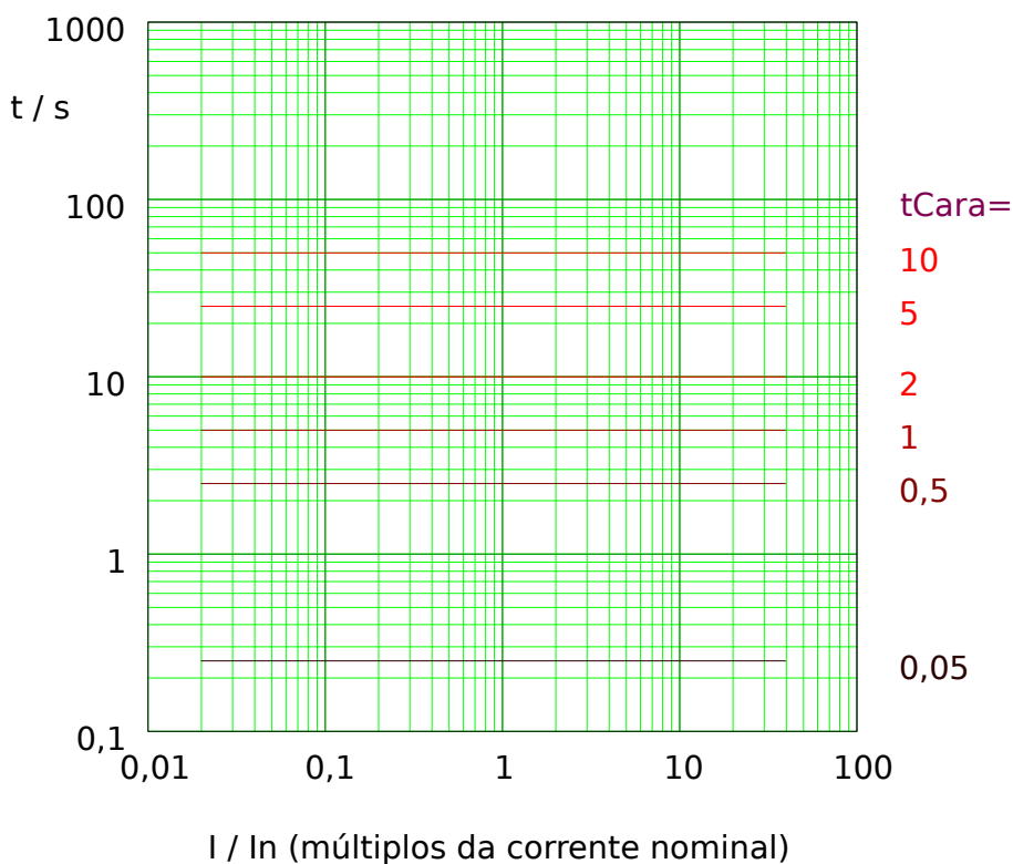
Fig. 85: Sup Térmi tripping curve. Note that only the range I \geq I> is actually effective.
