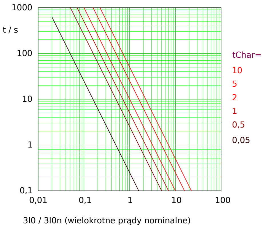
Rys. 91: I2T tripping curve. Note that only the range 3I0 \geq \text{Próg } 3I0 is actually effective.
