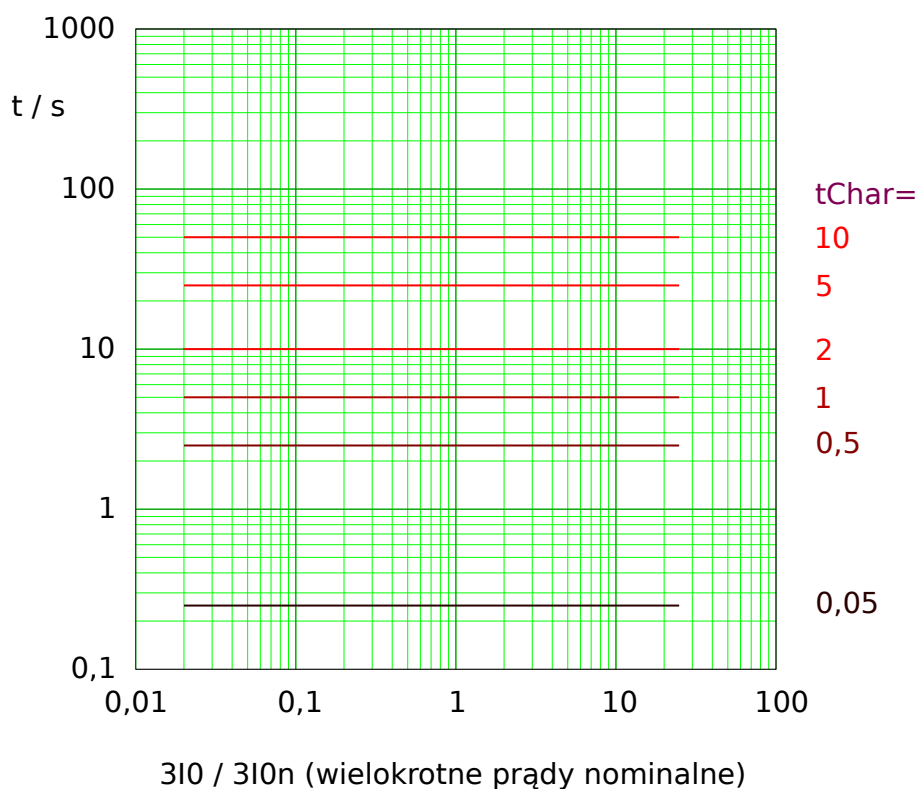
Rys. 89: Termiczna Płaska tripping curve. Note that only the range 3I0 \geq \text{Próg } 3I0 is actually effective.
