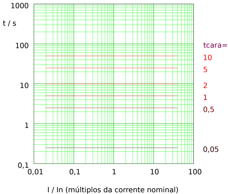
Fig. 85: Sup Térm tripping curve. Note that only the range I \geq I > is actually effective.
