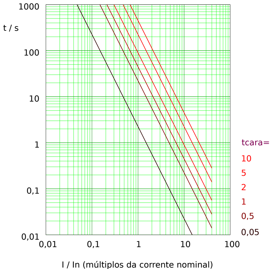
Fig. 87: I2T tripping curve. Note that only the range I \geq I_n is actually effective.
