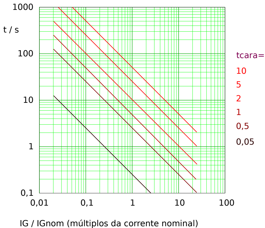
Fig. 90: IT tripping curve. Note that only the range IG \geq IG_{nom} is actually effective.
