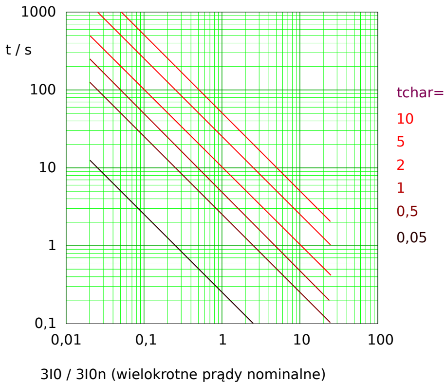
Rys. 90: IT tripping curve. Note that only the range 3I0 \geq \text{Próg } 3I0 is actually effective.
