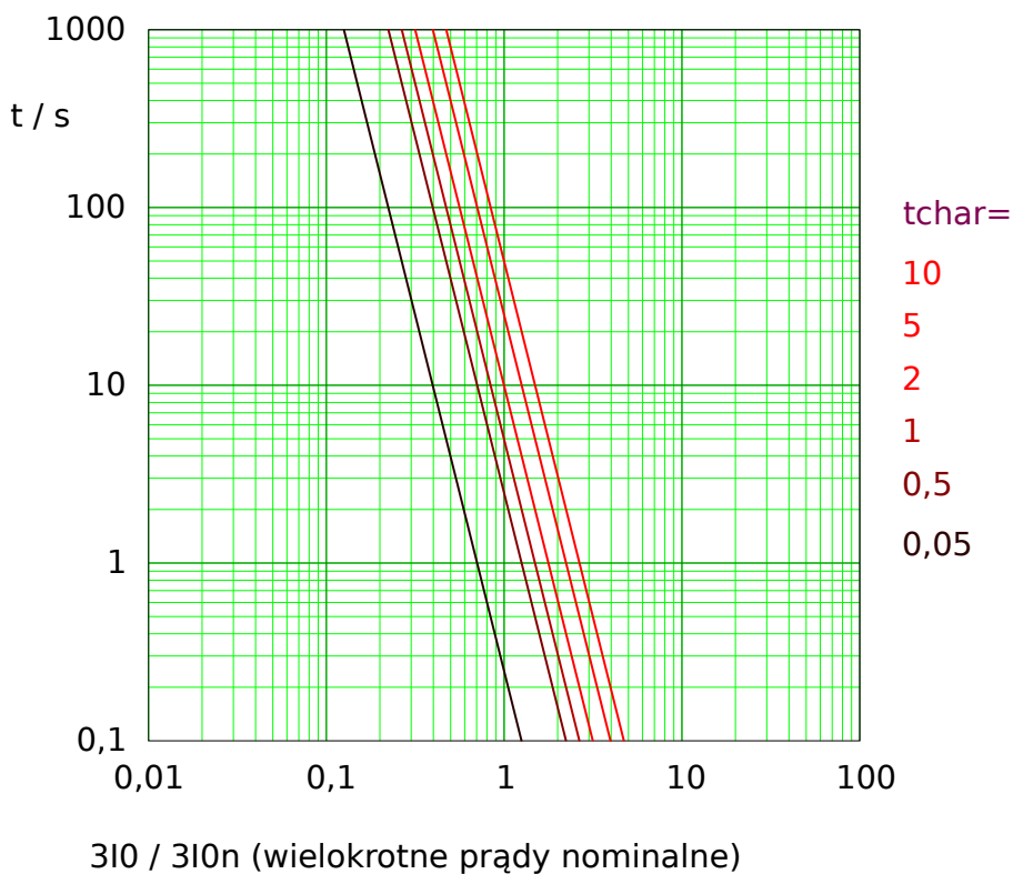
Rys. 92: I4T tripping curve. Note that only the range 3I0 \geq \text{Próg } 3I0 is actually effective.
