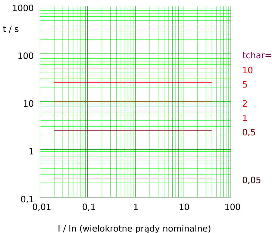
Rys. 85: Termiczna Płaska tripping curve. Note that only the range I \geq I> is actually effective.
