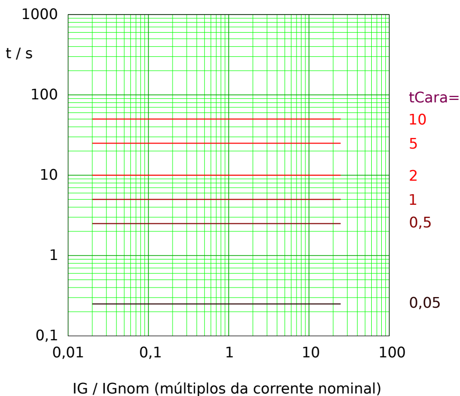
Fig. 75: Sup Térmi tripping curve. Note that only the range IG \geq IG> is actually effective.
