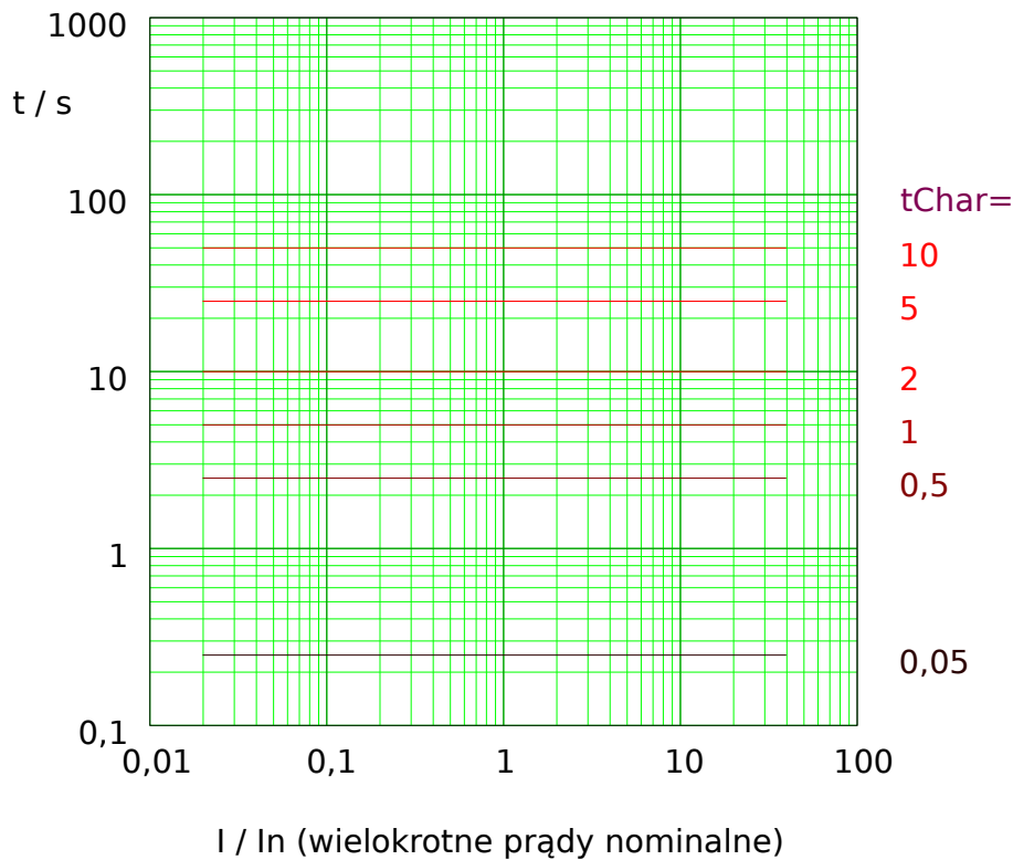
Rys. 71: Termiczna Płaska tripping curve. Note that only the range I \geq I > is actually effective.
