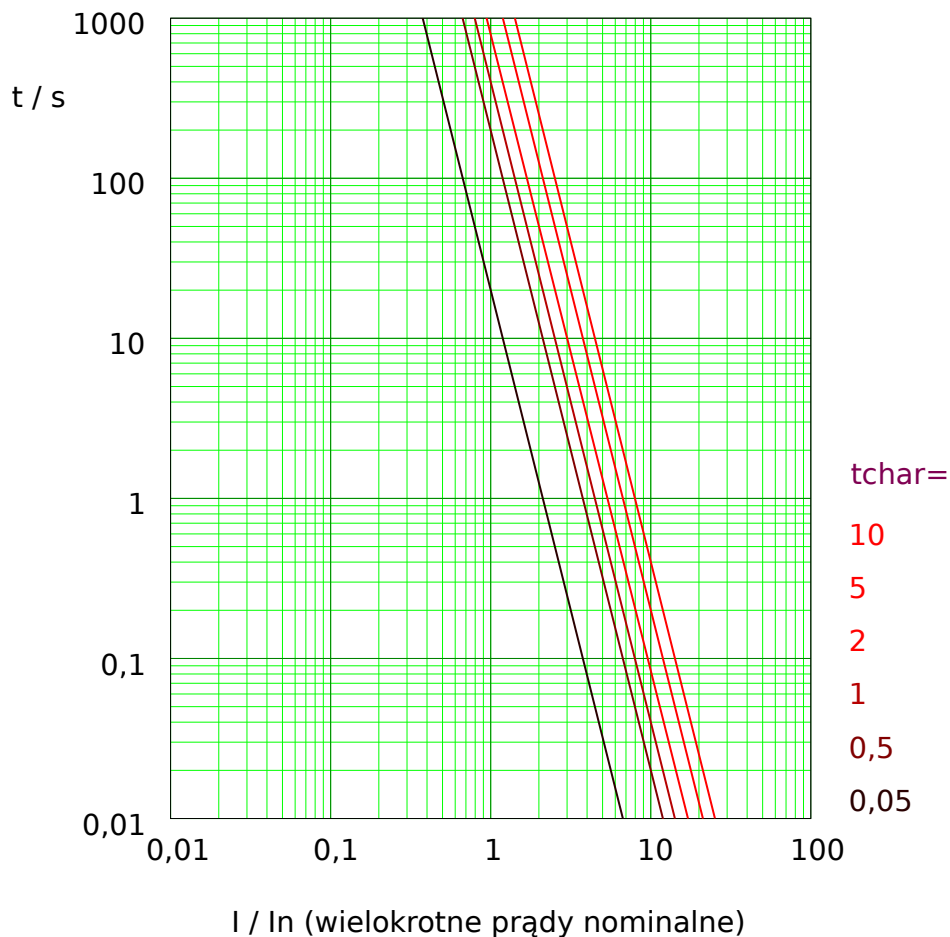
Rys. 74: I4T tripping curve. Note that only the range I \geq I > is actually effective.
