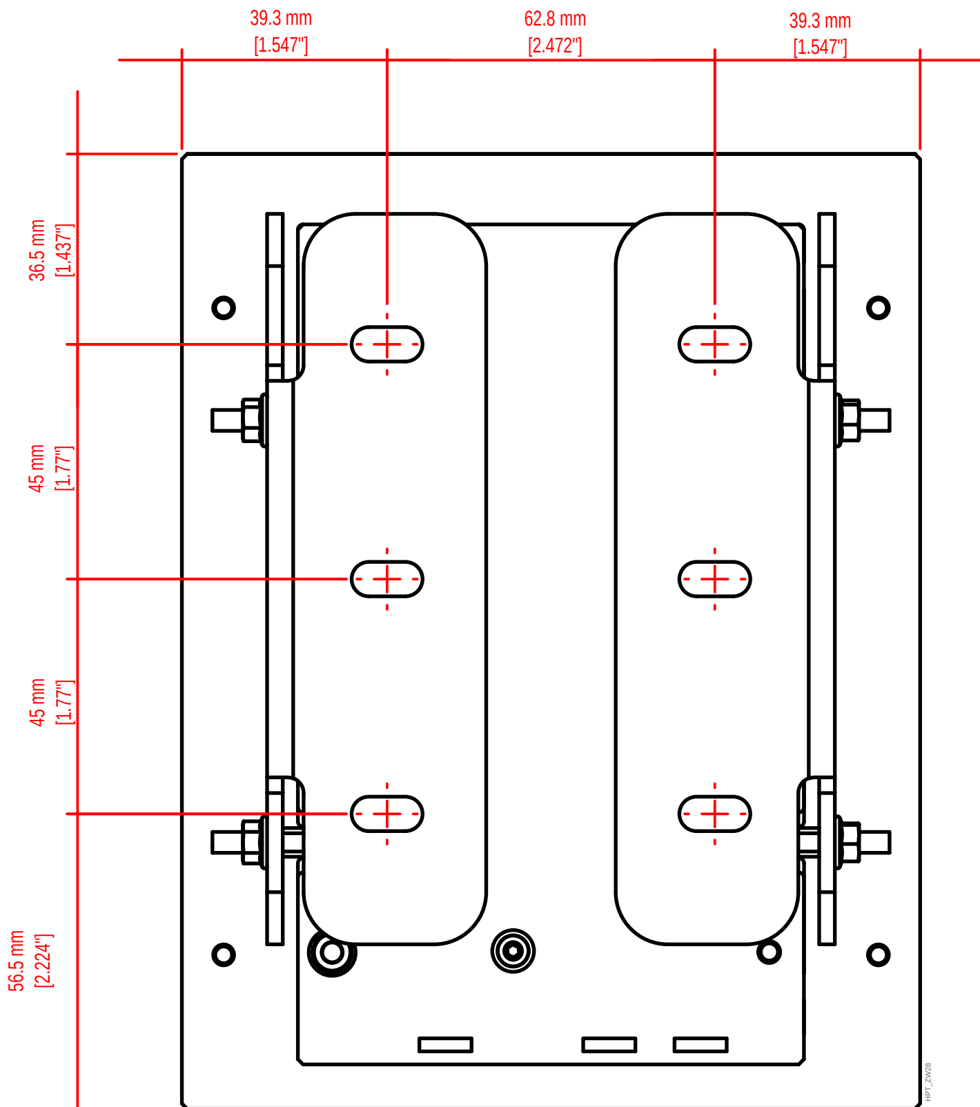
B1 Housing: back view Please print with scaling set to 100% and evaluate lengths afterwards.
