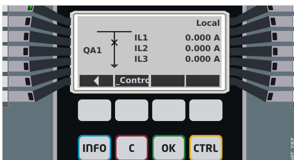
Fig. 4: Control Page Example, with the “Circuit Breaker” in closed position.
