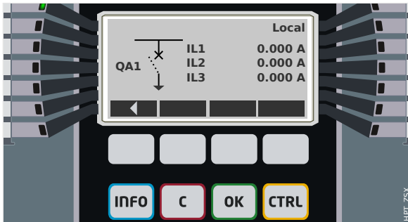
Fig. 3: Control Page Example, with the “Circuit Breaker” in intermediate position.
