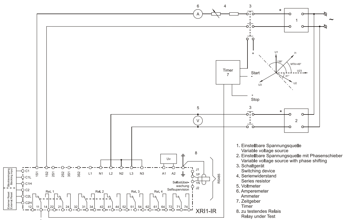
Figure 7.1: Test circuit
