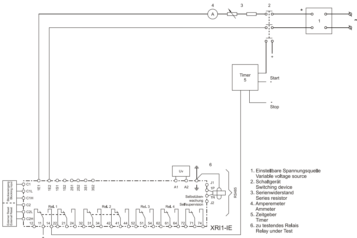
Figure 7.1: Test circuit
